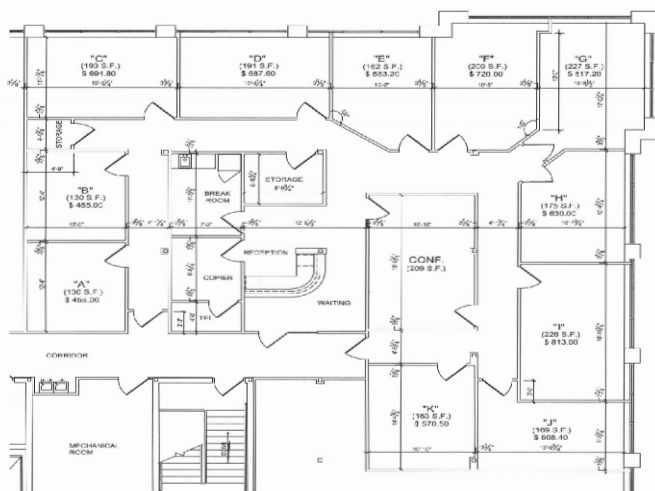
PARTIAL SECOND FLOOR PLAN - EXECUTIVE SUITES SCALE: 1/8" = 1'-0" TOWN CENTER TOWER EAST 9.9.09
